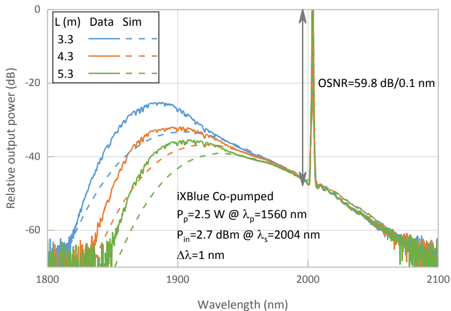
Figure 6: Output spectrum of the iXBlue co-pumped amplifier for different active fiber length.
