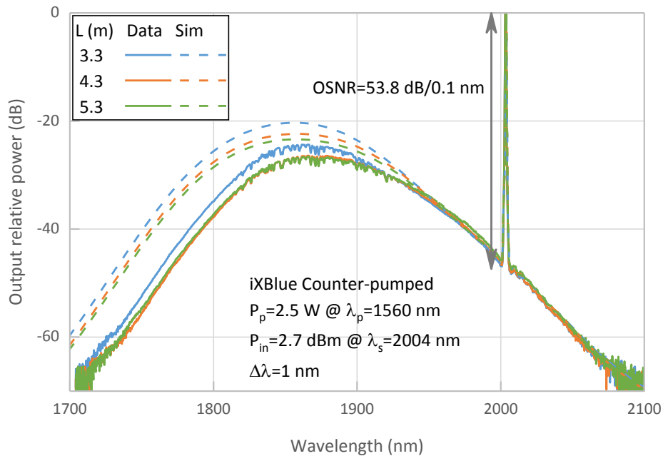
Figure 8: Output spectrum of the iXBlue counter-pumped amplifier for different active fiber length.
