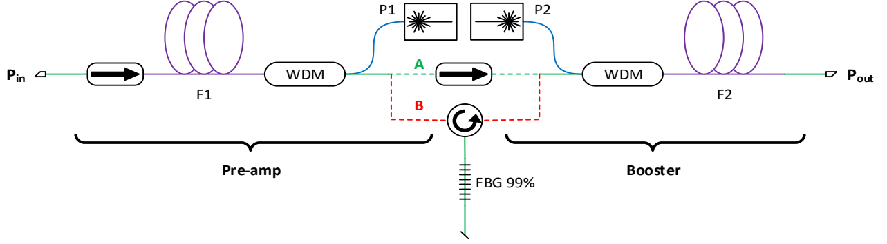
Figure 9: Topology of our two stage TDFA operating at 1952 nm.
