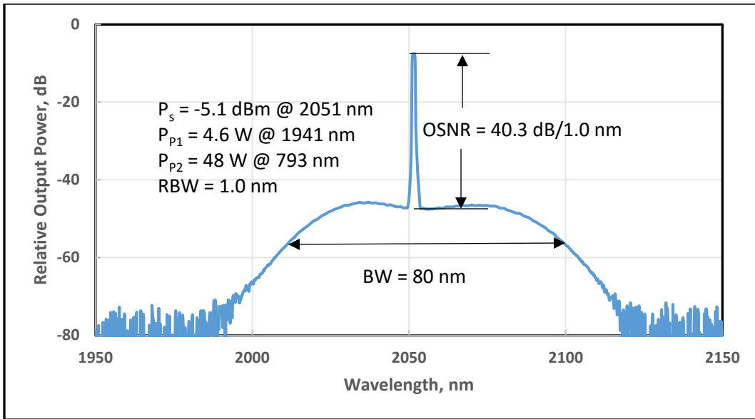
Figure 6. Output Optical Spectrum for P_s = -5 \text{ dBm} . RBW = 1.0 nm.
