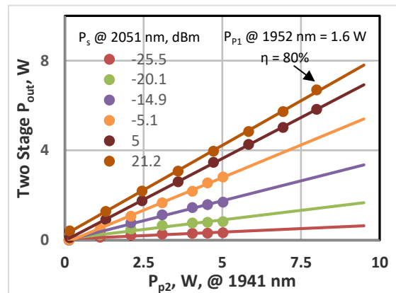
Figure 5. Two Stage P_{out} vs. P_{p2} for Different P_s Levels
