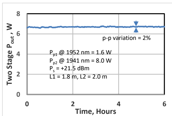
Figure 8. Long-Term Stability of P_{out} .
