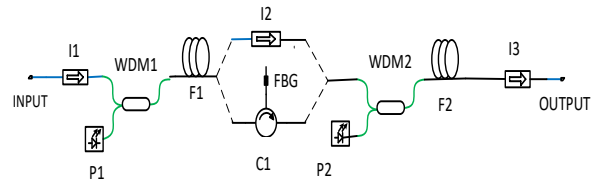
Figure 1. Two Stage PM HDFFA with Multiwatt Pump Sources in the 1950 nm Band
