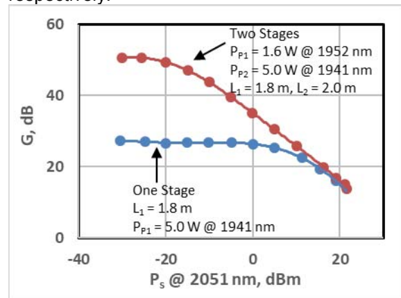
Figure 6. G vs. P_s for One and Two Stages with Different P_p Levels
