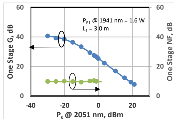
Figure 2. G and NF for One Stage High Gain PM HDFFA
