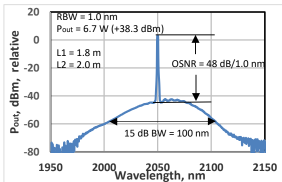
Figure 9. Saturated Output Spectrum of the Two Stage High Power HDFAs.
