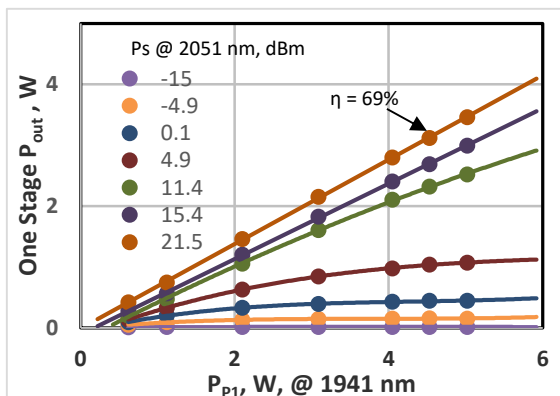
Figure 4. One Stage P_{out} vs. P_{p1} for Different P_s Levels
