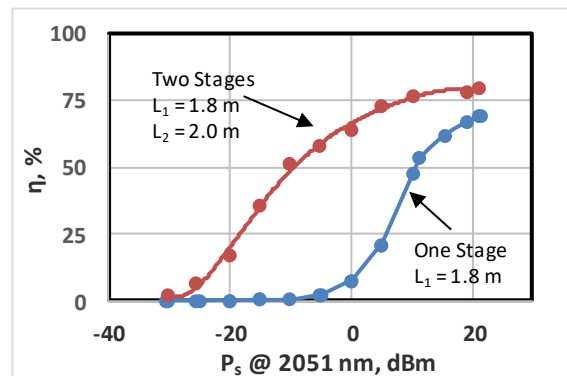
Figure 7. \eta vs. P_s for One and Two Stage Configurations
