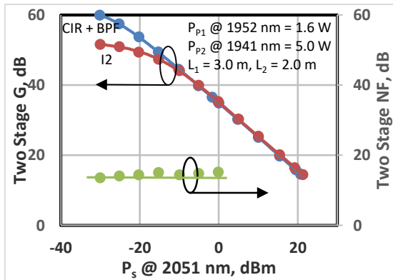
Figure 3. G and NF for Two Stage High Gain PM HDFA
