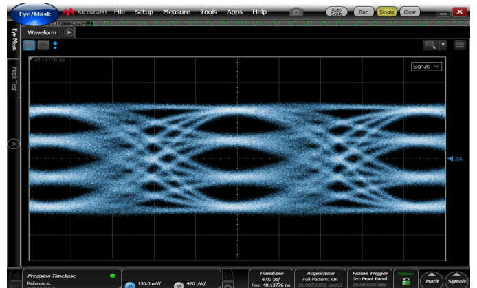
28 Gbauds PAM-4 eye diagram
