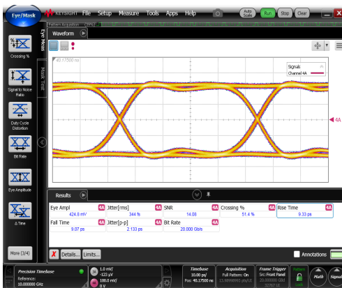
Input signal Eye amplitude = 0.43 V pp
