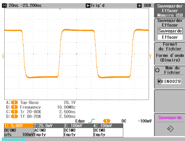
Width = 20 ns
