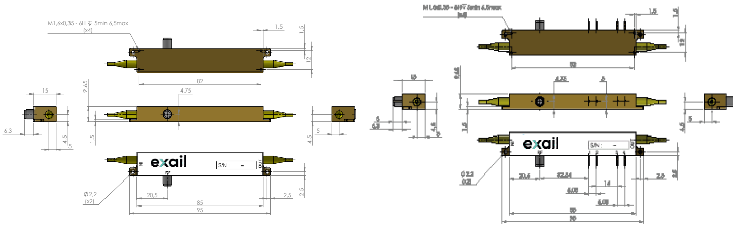
Housing #A: Standard Modulator housing
